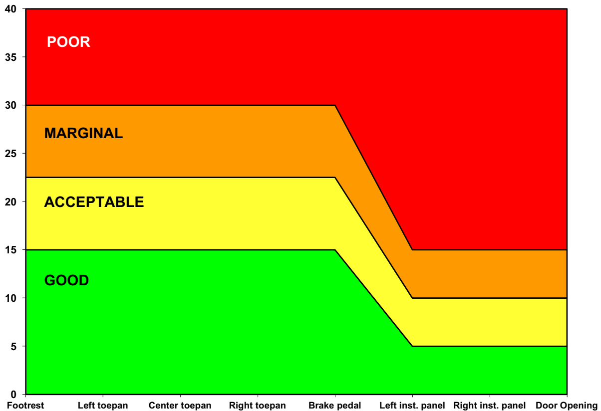
Figure 1 Guidelines for Rating Occupant Compartment Intrusion (cm)
